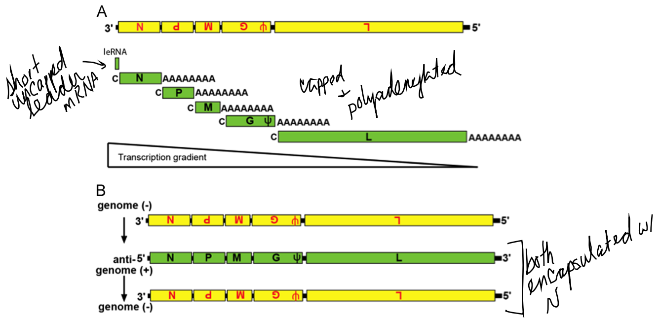
Fig. 3. Transcription and replication of a NNSV shown for RABV. (A) The encapsidated negative-strand RNA (yellow) serves as a template for the polymerase complex. Transcription starts with a short uncapped leader RNA (leRNA) from the 3' end of the genomic RNA; this is followed by the transcription of 5' capped and polyadenylated mRNAs, which encode the viral proteins (green). The polymerase complex stops at a signal sequence, ignores the intergenic region (IGR) and restarts transcription at the transcription start signal sequence. Subsequent attempts at transcription by the polymerase complex are not always successful; therefore, attenuation of transcription occurs in the direction of 3'-5' (transcription gradient). (B) During replication, the polymerase complex ignores the transcription start/stop signals within the RABV genome (yellow), rendering a full-length antigenomic RNA (green), which is also encapsidated. The antigenomic RNA is encapsidated into the N protein along with the genomic RNA. The synthesized antigenome serves then as a template for the synthesis of additional copies of genomic RNA (yellow). (For interpretation of the references to color in this figure legend, the reader is referred to the web version of this article.)
